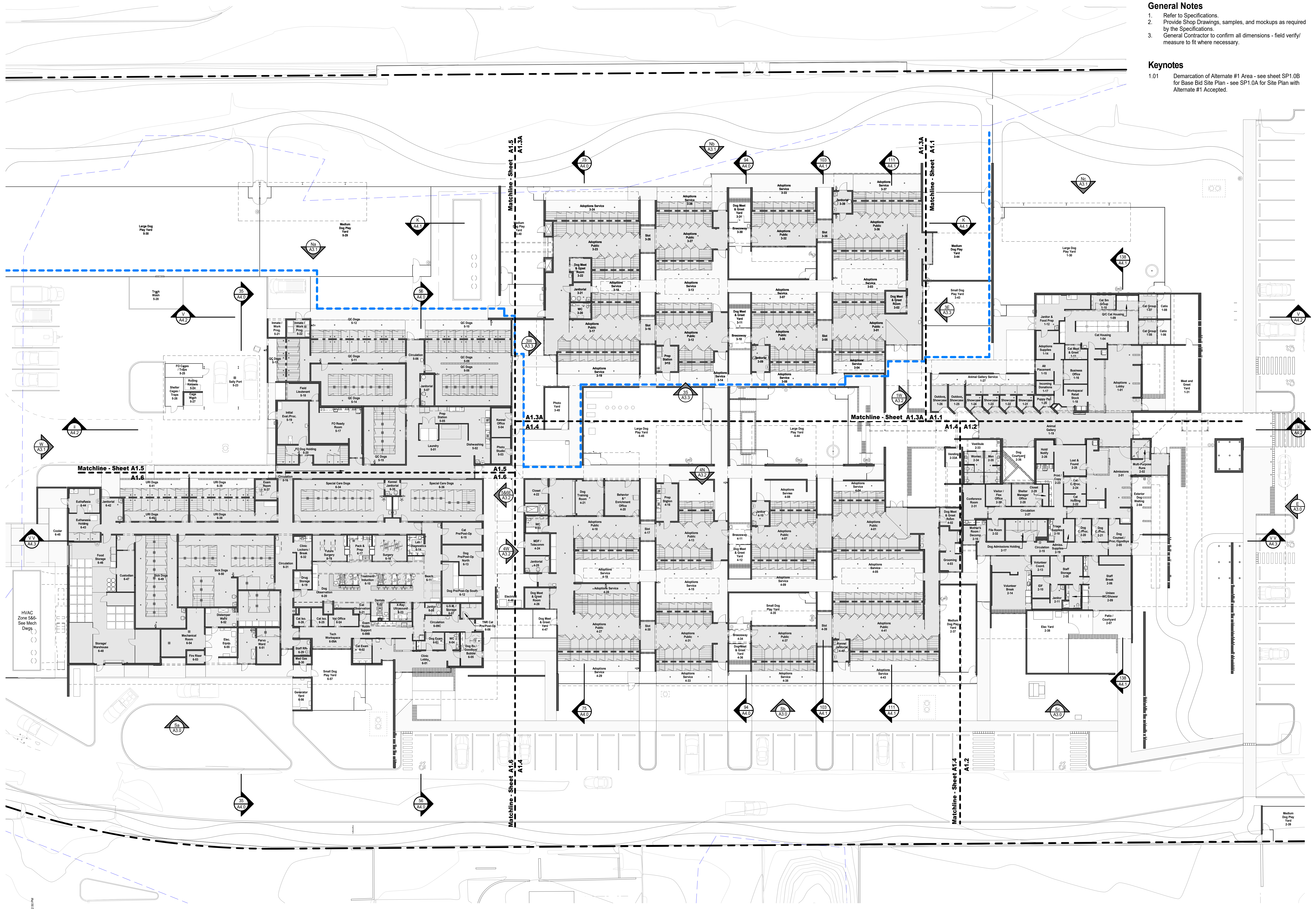
1 Overall Floor Plan - All Zones (with Alternate #1 Accepted)
