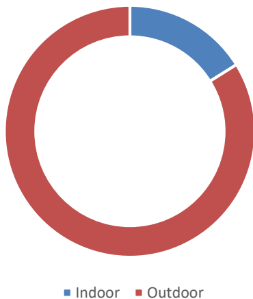
Graph 2. 84% of heat-associated deaths have had an injury place outdoors.
