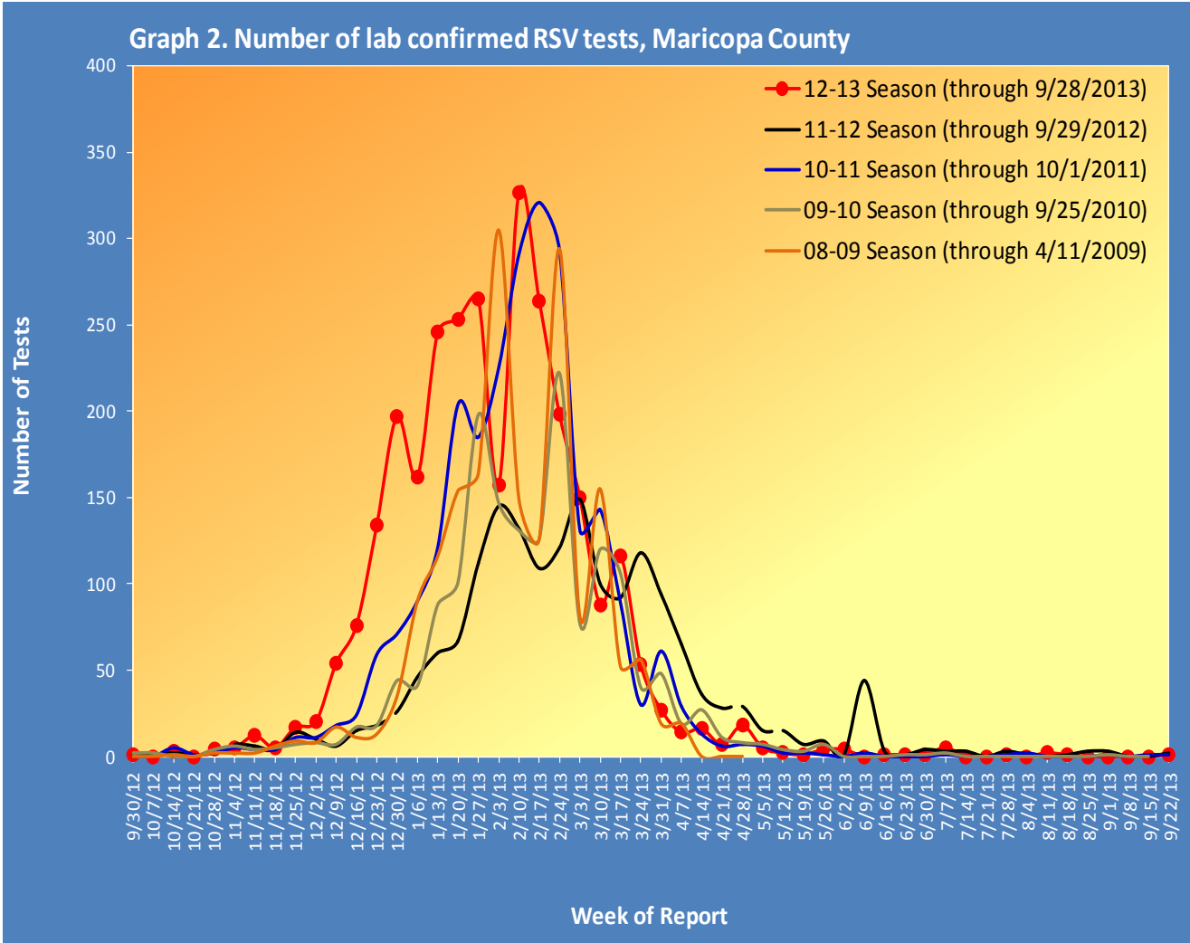
Graph 2 shows confirmed RSV tests for the current season (red) and previous seasons.
